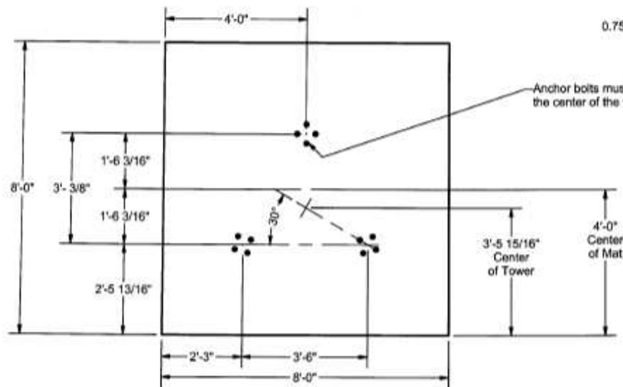
PLAN VIEW (Reinforcement not shown for clarity)
